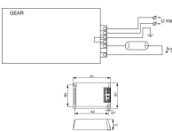
Scheda tecnica Philips HID-PV C 70 /S CDM 220-240V 50/60Hz
